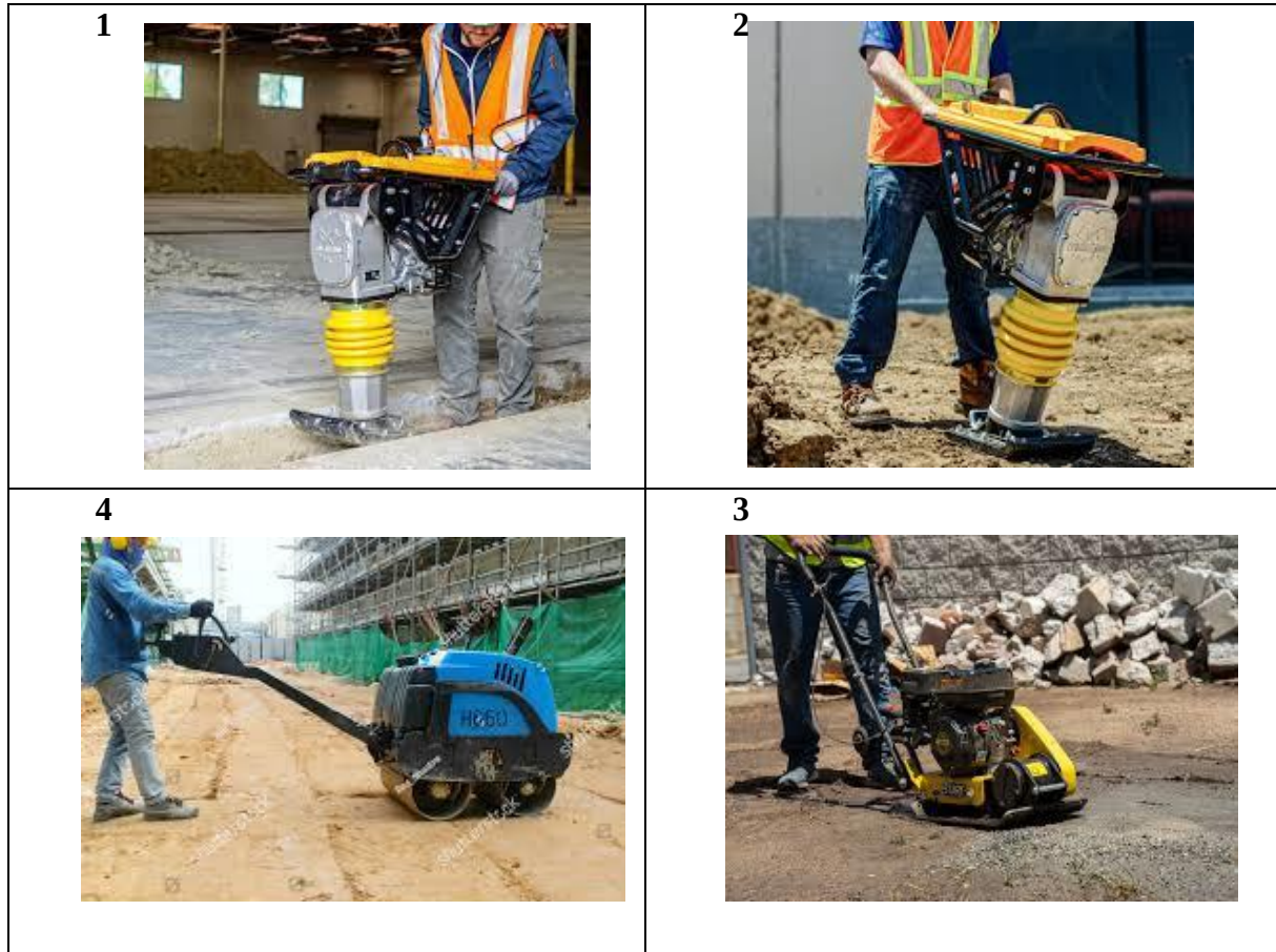
Figure 1. Specialized Equipment for Confined Areas.1- Handheld Tampers. 2- Jumping Jack Rammers. 3- Walk-Behind Plate Compactors.4- walk-behind roller compactors.
