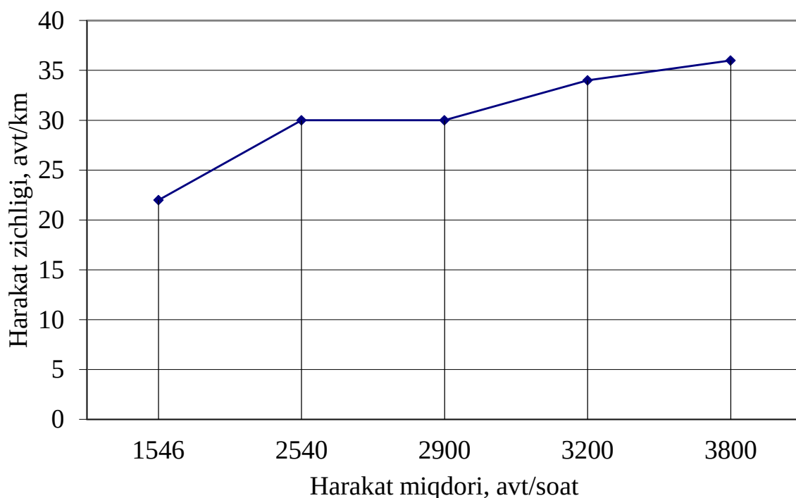
2-rasm. I.Karimov ko'chasida harakat zichligining o'zgarishi.
