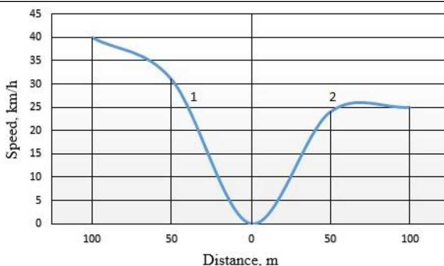
Figure 5. Speed graph provided by distances from the entrance and exit to the parking area Entrance to parking lot 1; exit from parking lot 2.
