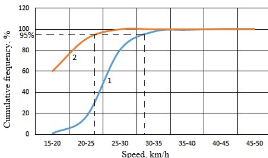
Figure 2. Cumulative curvature graph Entrance to parking lot 1; exit from parking lot 2.
